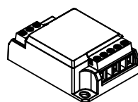
SPD CL.I 12KV 320V UC max 40x57x20mm code 9058
