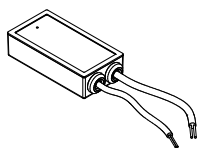
Power supply 16W 220-240V IP65 125x61x31mm
