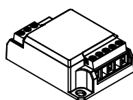
SPD CL.1 12KV 320V UC max 40x57x20mm
