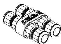
3-4 way - 4 poles terminal block IP68 53x26x82mm code 9005
