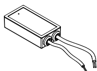
Power supply 16W220-240 IP65 125x61x31mm code 9059
